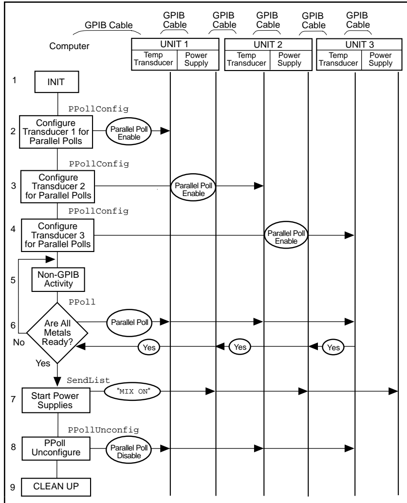
Figure 2-8. Program Flowchart for Example 8
