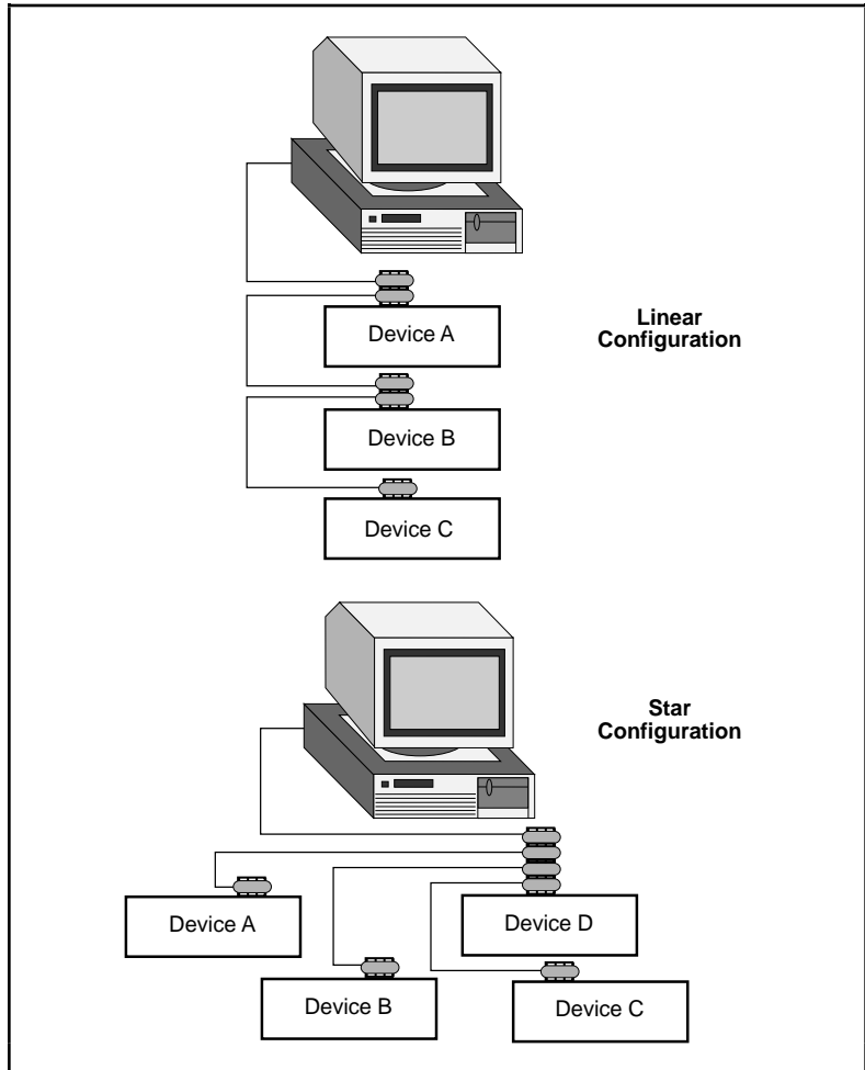
Figure 1-2. Linear and Star System Configuration
