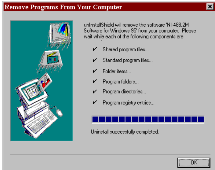
Figure 1-7. Uninstallation Results
